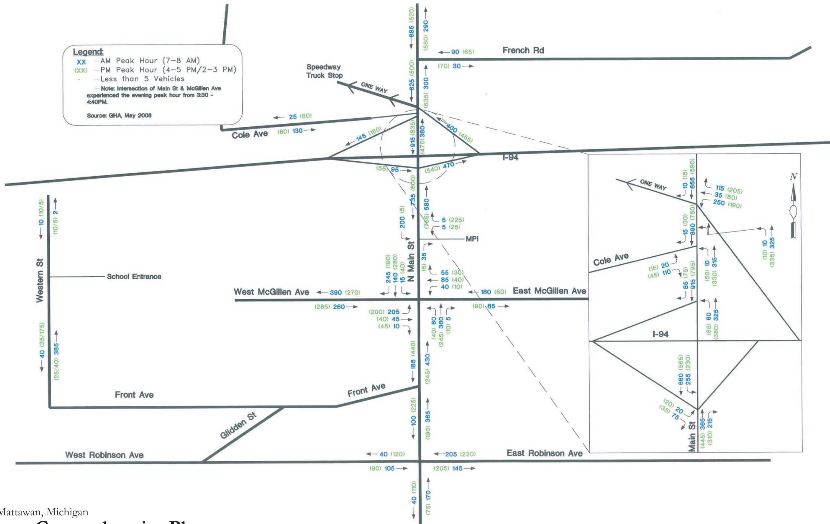
Figure 5.3: Existing Peak Traffic Volumes
